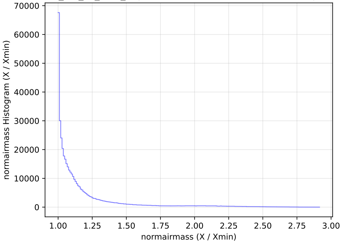
mw_roll_all_v3.3_10yrs WFD z band: normairmass Histogram
