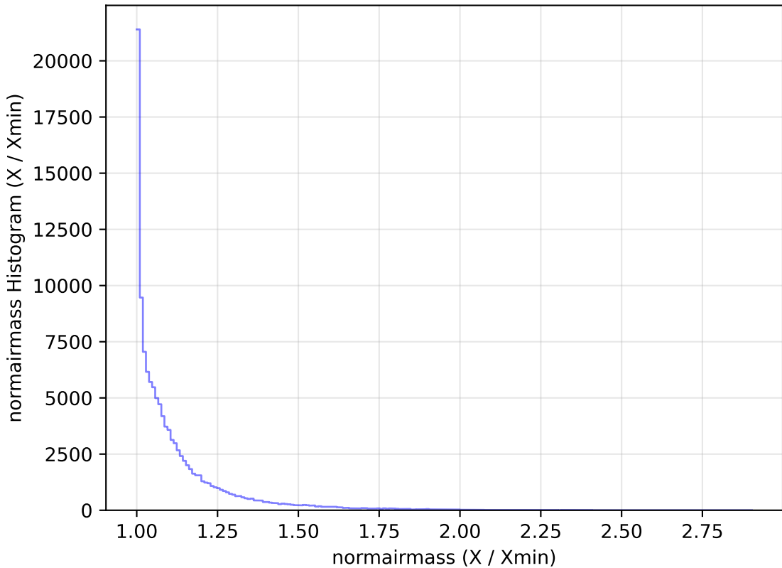
mw_roll_all_v3.3_10yrs WFD u band: normairmass Histogram
