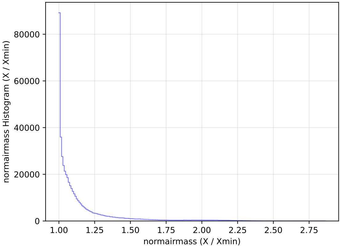
mw_roll_all_v3.3_10yrs WFD r band: normairmass Histogram
