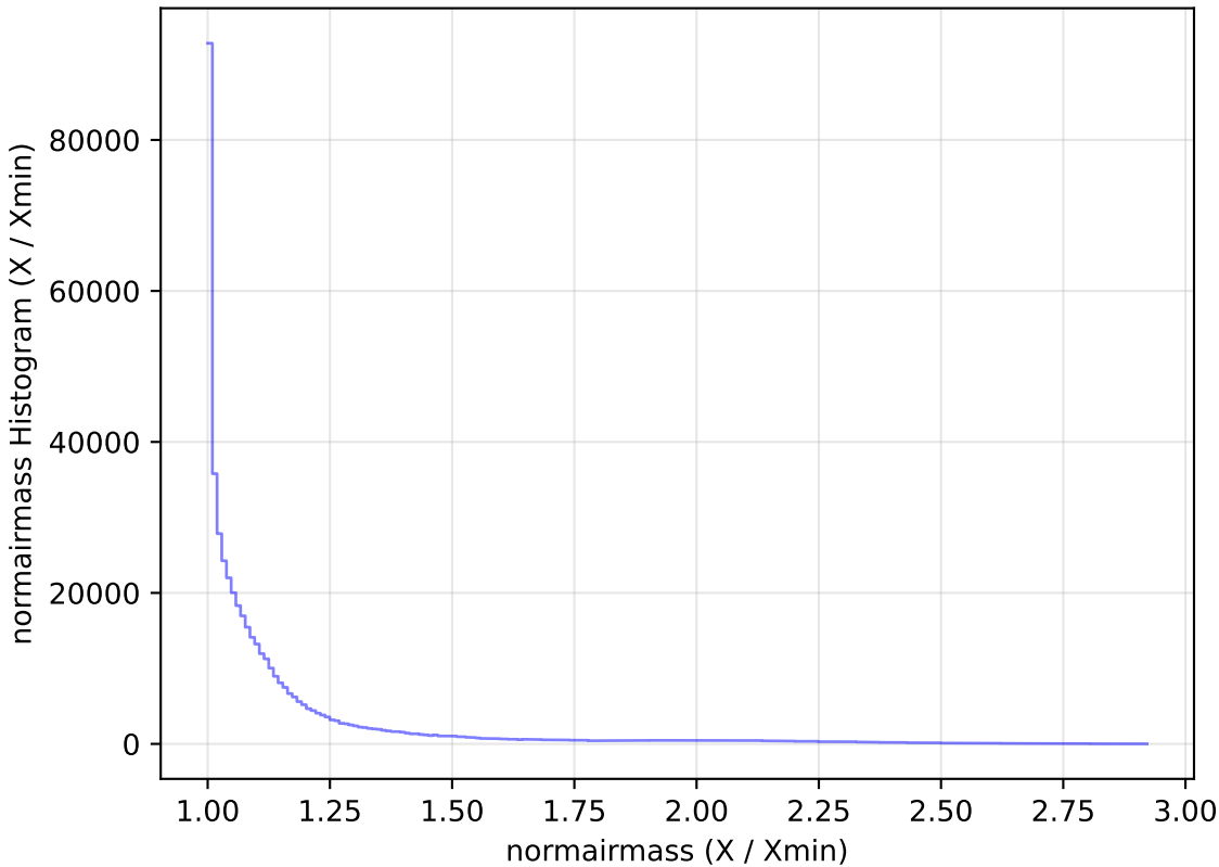
mw_roll_all_v3.3_10yrs WFD i band: normairmass Histogram
