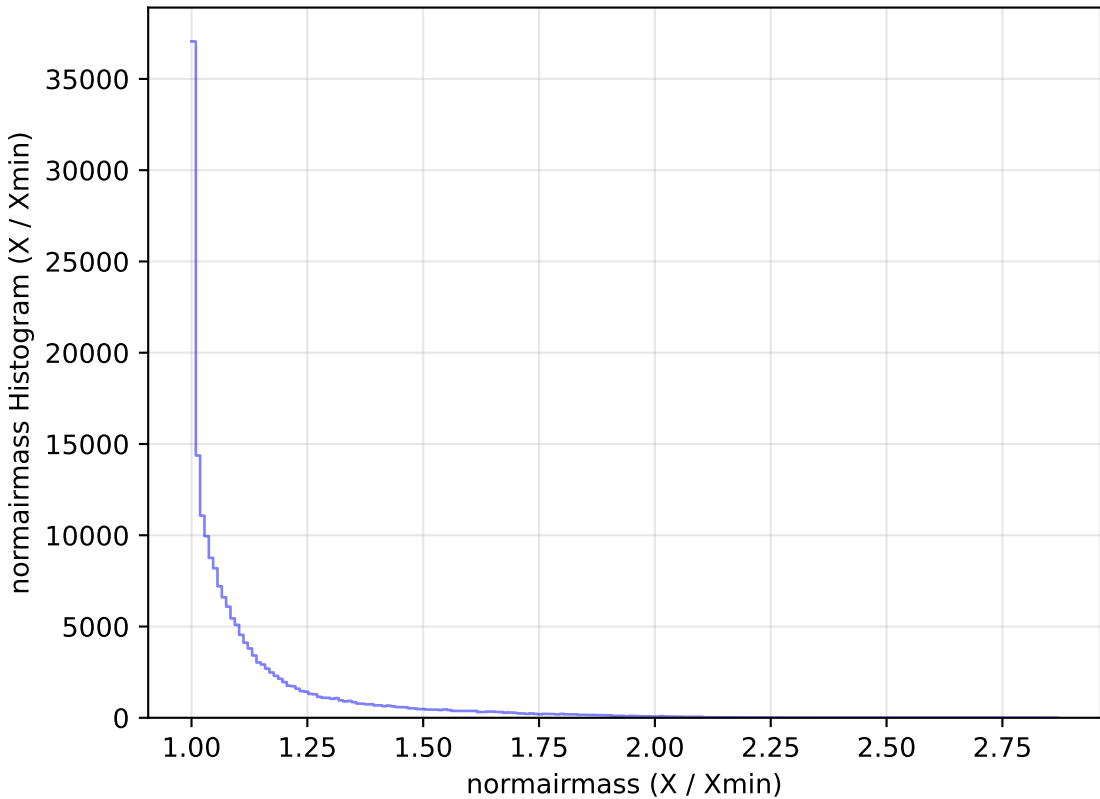
mw_roll_all_v3.3_10yrs WFD g band: normairmass Histogram
