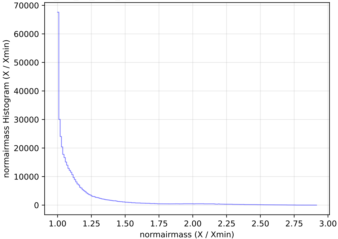
mw_roll_all_v3.3_10yrs All sky z band: normairmass Histogram
