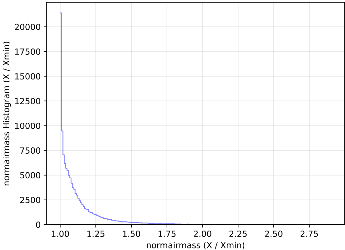
mw_roll_all_v3.3_10yrs All sky u band: normairmass Histogram
