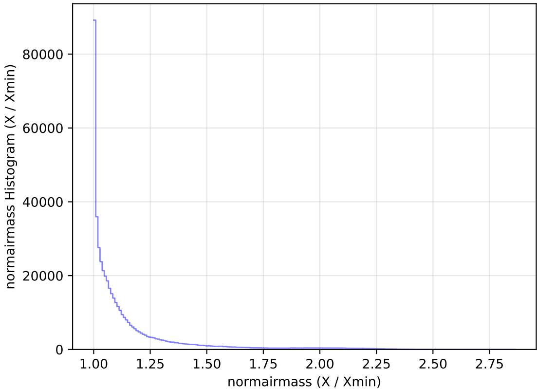
mw_roll_all_v3.3_10yrs All sky r band: normairmass Histogram
