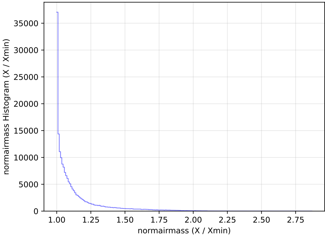
mw_roll_all_v3.3_10yrs All sky g band: normairmass Histogram
