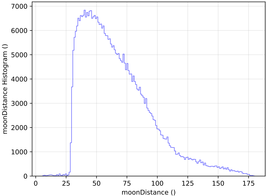
mw_roll_all_v3.3_10yrs WFD y band: moonDistance Histogram
