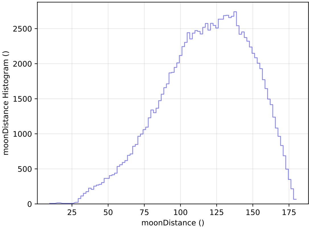
mw_roll_all_v3.3_10yrs WFD u band: moonDistance Histogram
