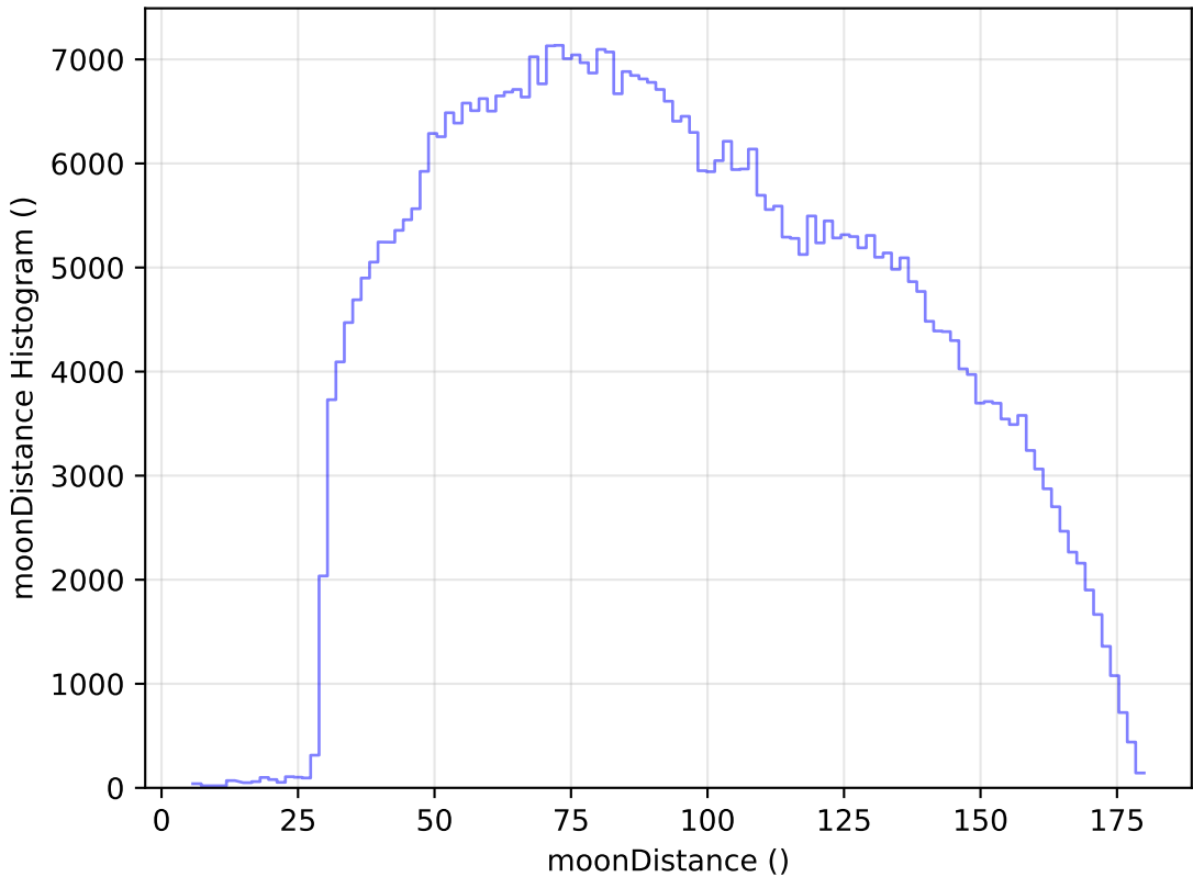
mw_roll_all_v3.3_10yrs WFD i band: moonDistance Histogram
