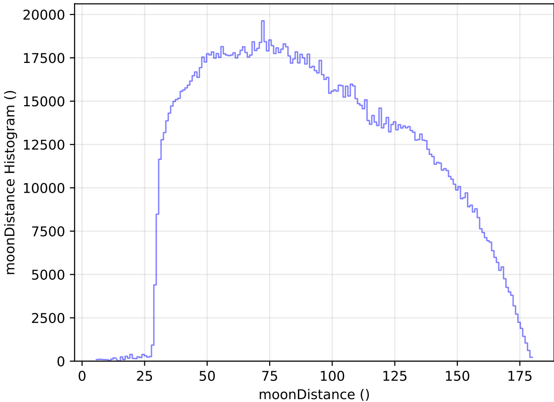
mw_roll_all_v3.3_10yrs WFD all bands: moonDistance Histogram
