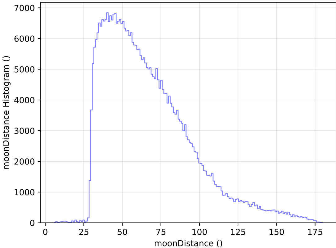
mw_roll_all_v3.3_10yrs All sky y band: moonDistance Histogram
