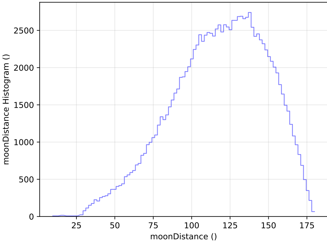
mw_roll_all_v3.3_10yrs All sky u band: moonDistance Histogram
