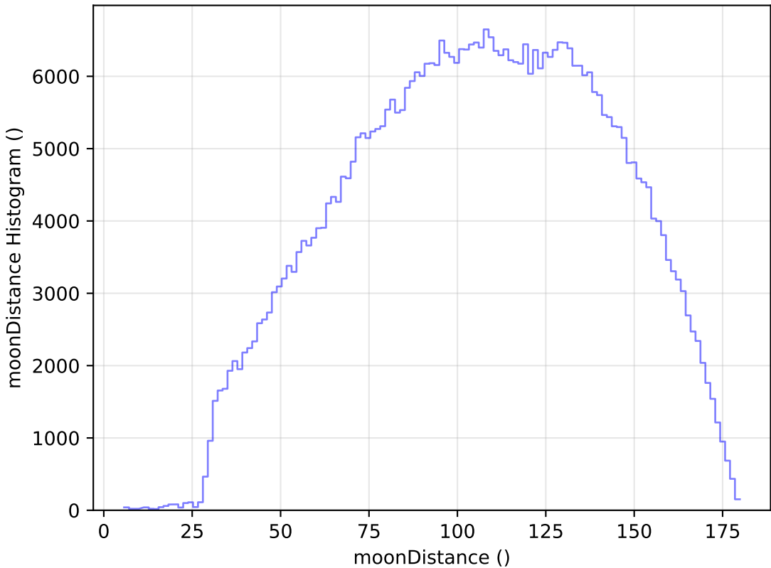
mw_roll_all_v3.3_10yrs All sky r band: moonDistance Histogram
