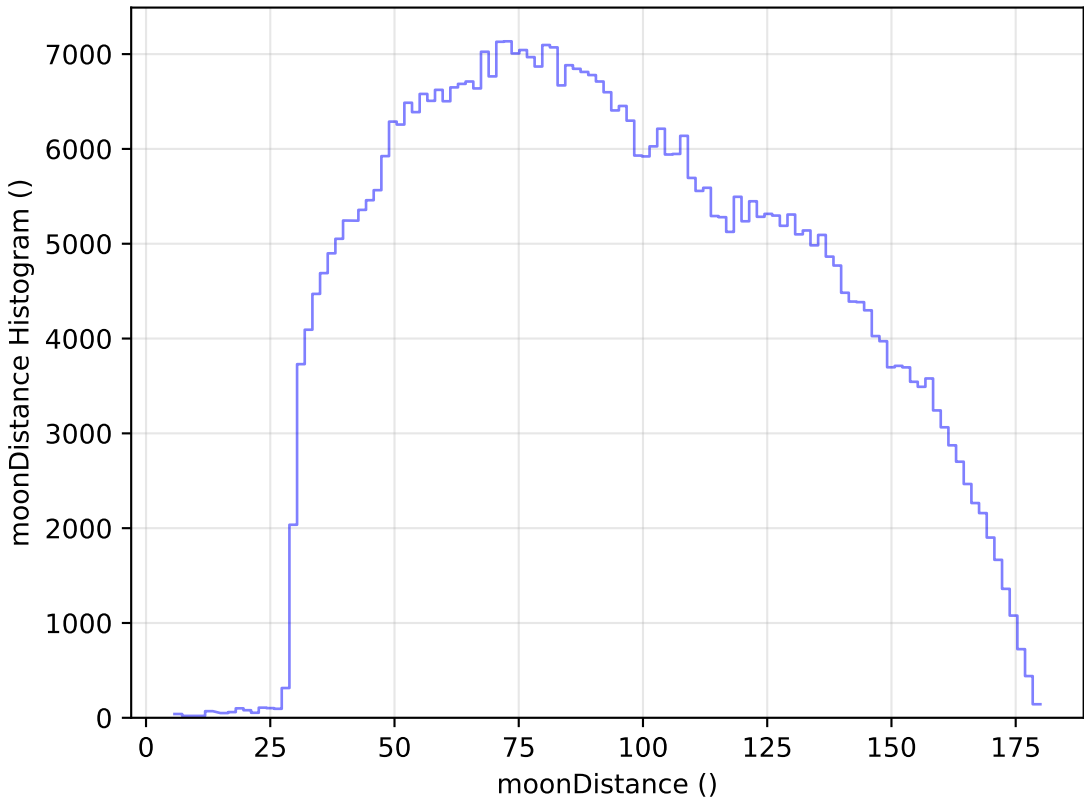
mw_roll_all_v3.3_10yrs All sky i band: moonDistance Histogram
