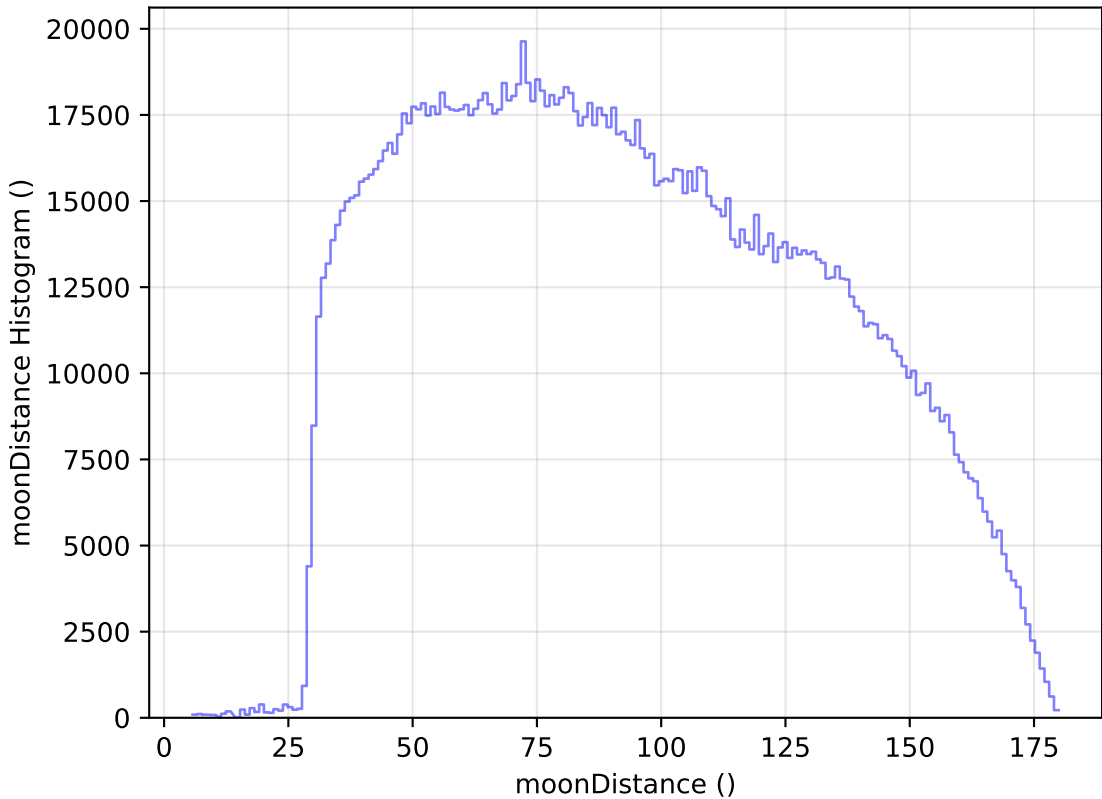
mw_roll_all_v3.3_10yrs All sky all bands: moonDistance Histogram
