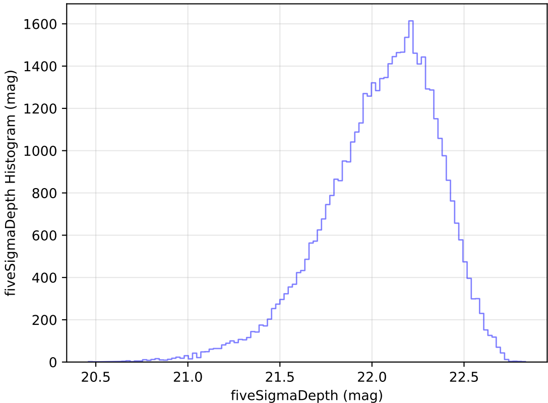
mw_roll_all_v3.3_10yrs Yr 1 y band: fiveSigmaDepth Histogram
