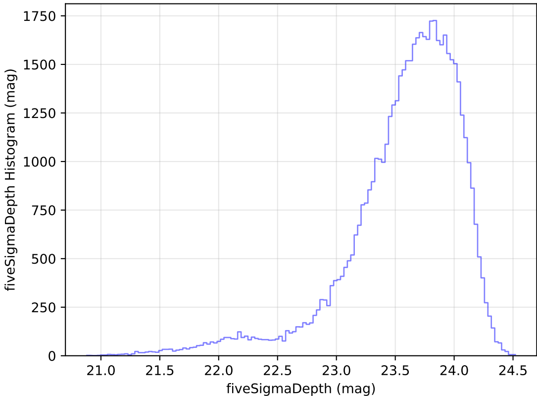
mw_roll_all_v3.3_10yrs Yr 1 i band: fiveSigmaDepth Histogram
