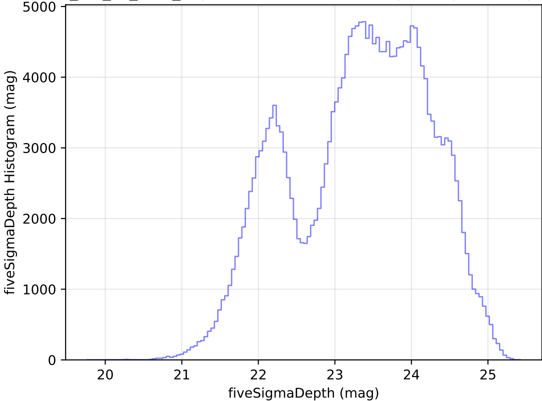
mw_roll_all_v3.3_10yrs Yr 1 all bands: fiveSigmaDepth Histogram
