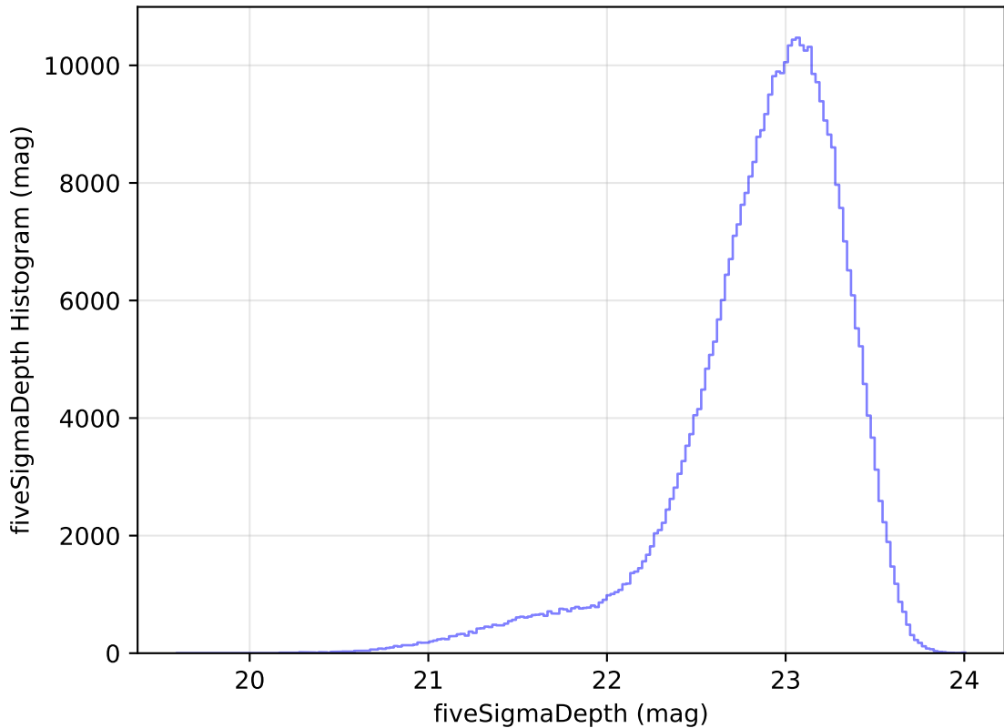
mw_roll_all_v3.3_10yrs WFD z band: fiveSigmaDepth Histogram
