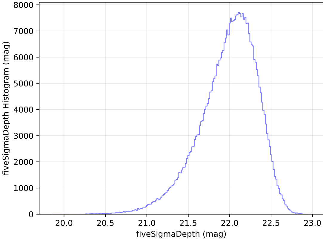
mw_roll_all_v3.3_10yrs WFD y band: fiveSigmaDepth Histogram
