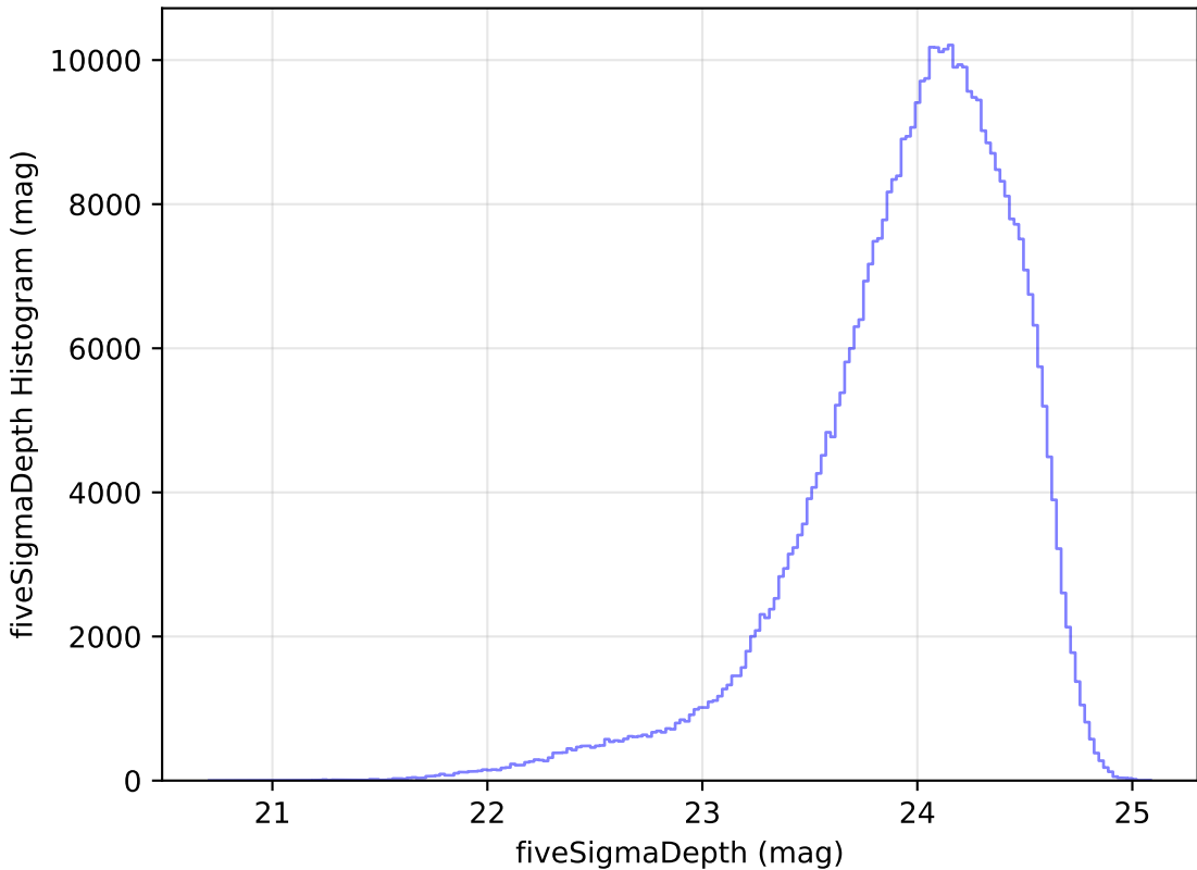
mw_roll_all_v3.3_10yrs WFD r band: fiveSigmaDepth Histogram
