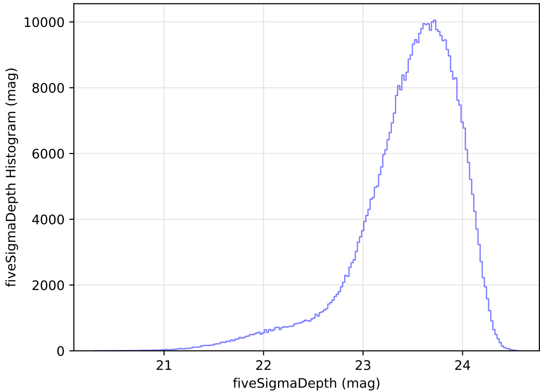
mw_roll_all_v3.3_10yrs WFD i band: fiveSigmaDepth Histogram
