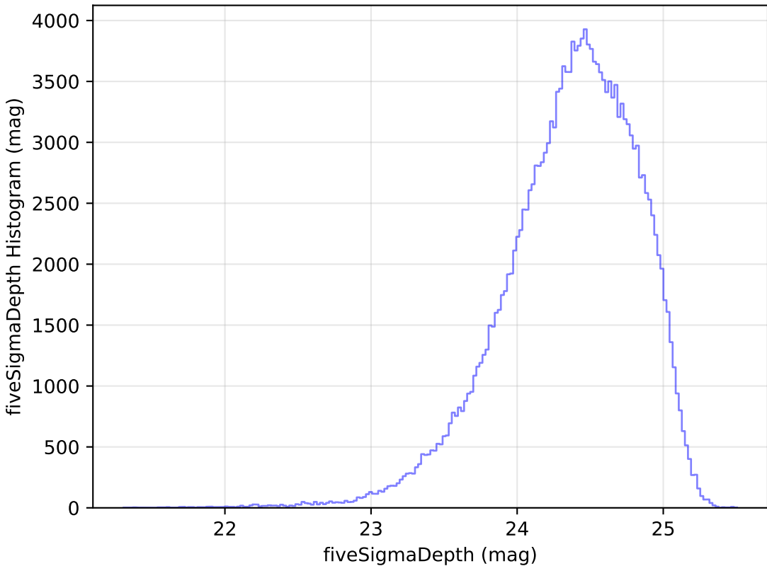
mw_roll_all_v3.3_10yrs WFD g band: fiveSigmaDepth Histogram
