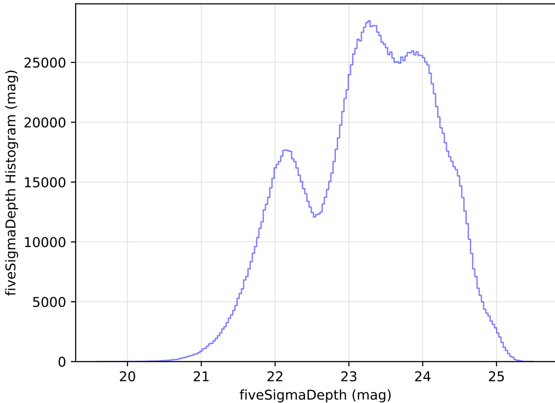
mw_roll_all_v3.3_10yrs WFD all bands: fiveSigmaDepth Histogram
