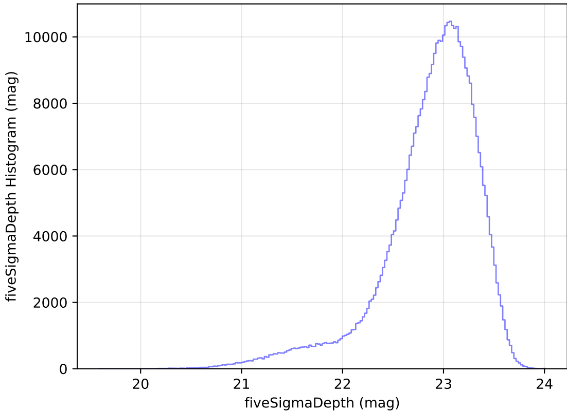
mw_roll_all_v3.3_10yrs All sky z band: fiveSigmaDepth Histogram
