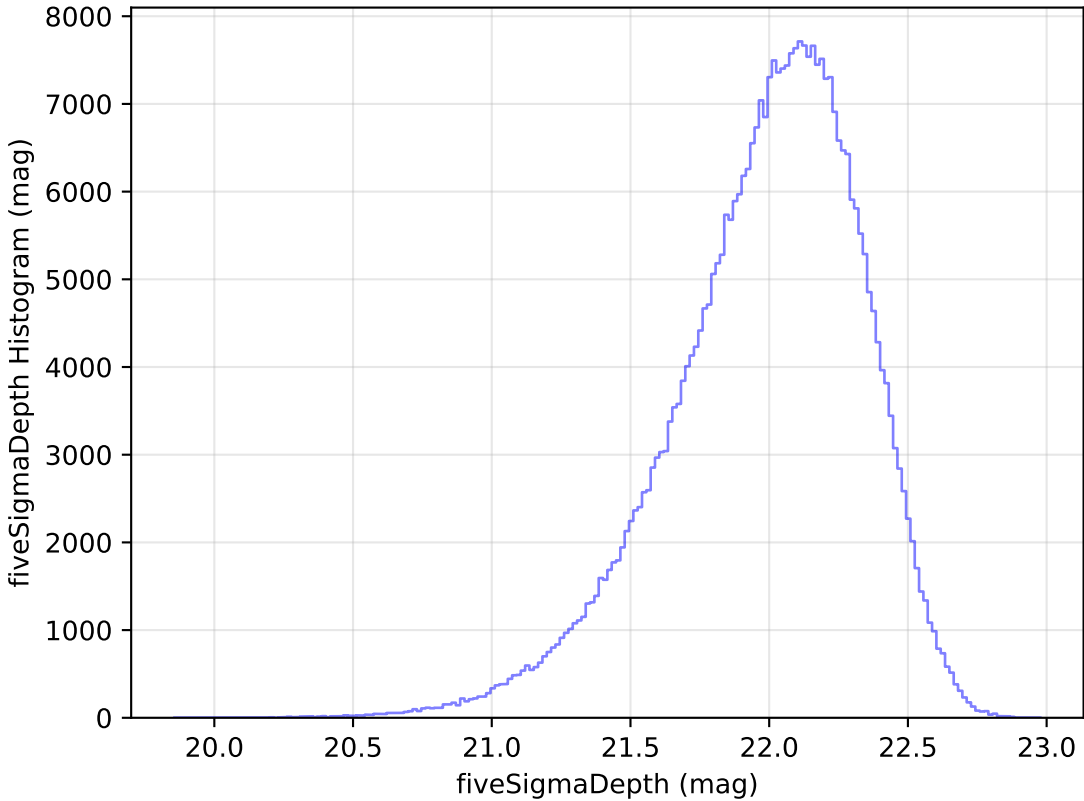
mw_roll_all_v3.3_10yrs All sky y band: fiveSigmaDepth Histogram
