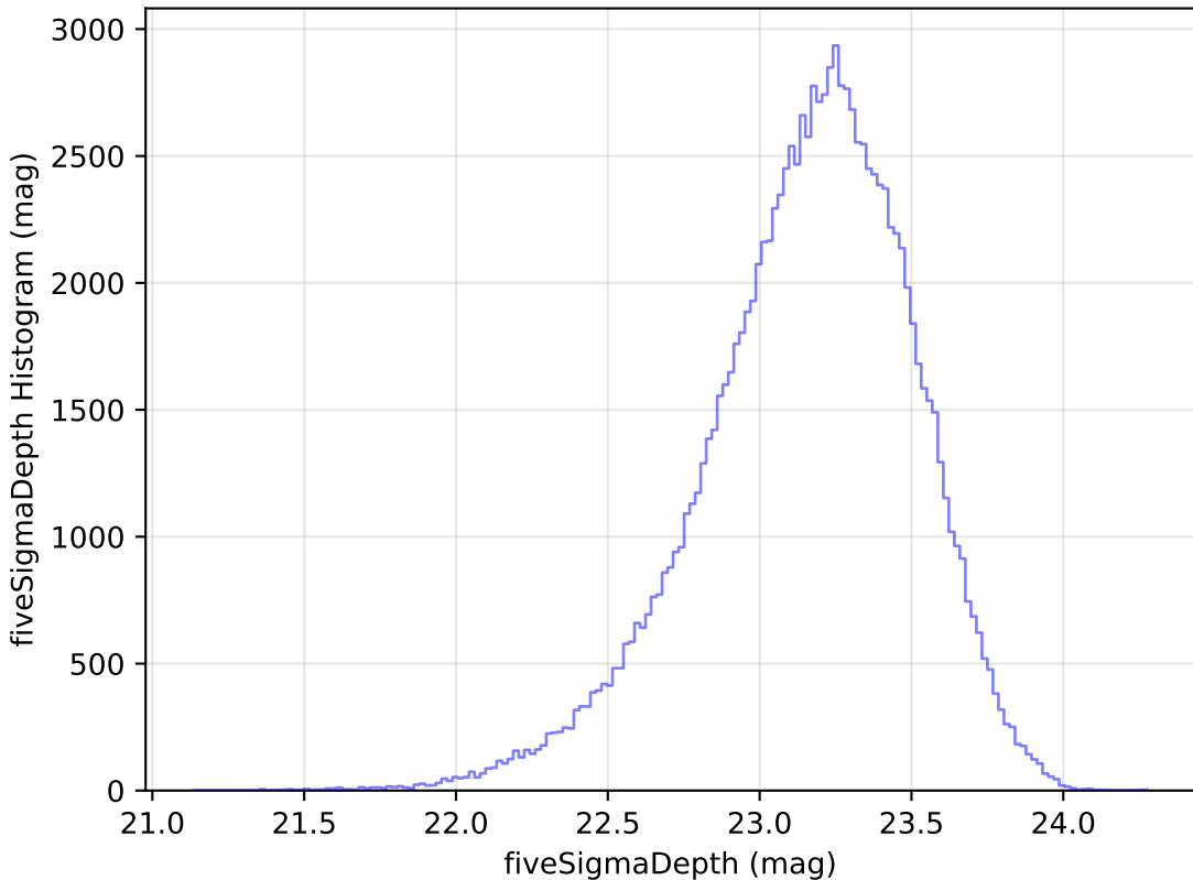
mw_roll_all_v3.3_10yrs All sky u band: fiveSigmaDepth Histogram
