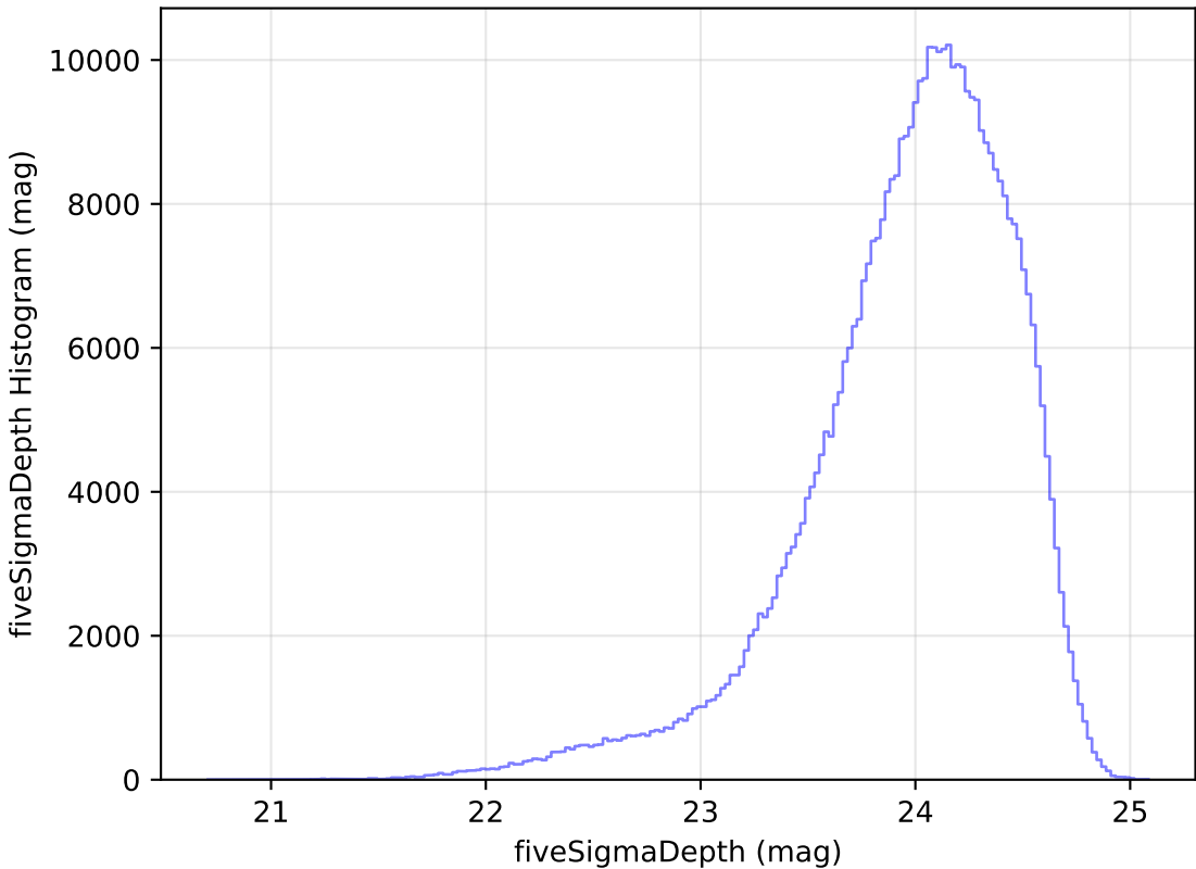
mw_roll_all_v3.3_10yrs All sky r band: fiveSigmaDepth Histogram
