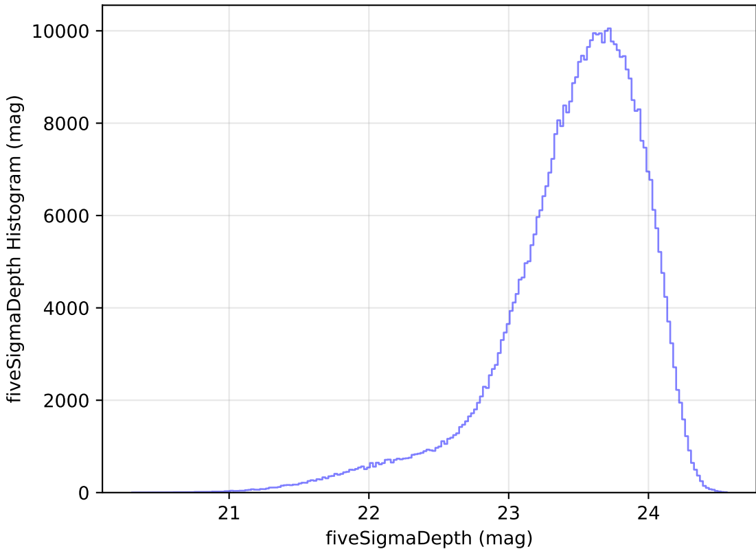
mw_roll_all_v3.3_10yrs All sky i band: fiveSigmaDepth Histogram
