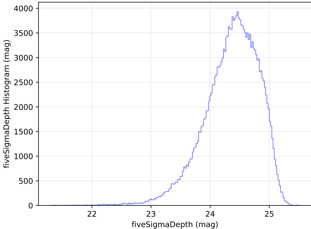
mw_roll_all_v3.3_10yrs All sky g band: fiveSigmaDepth Histogram
