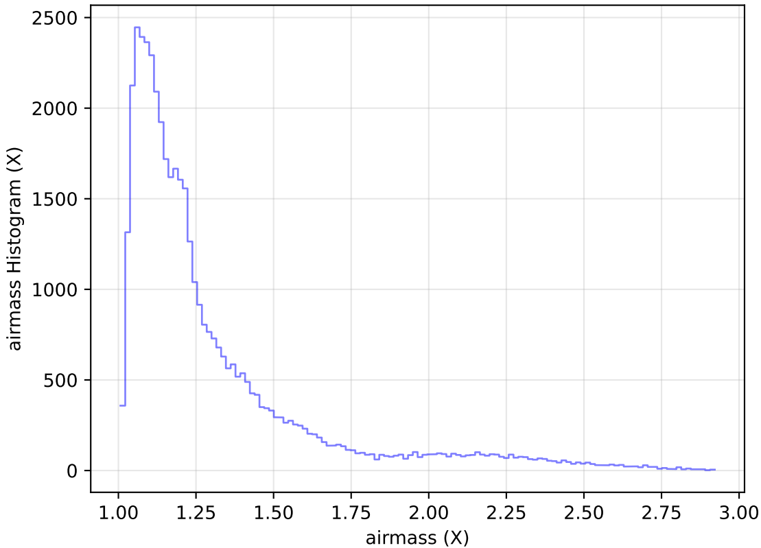
mw_roll_all_v3.3_10yrs Yr 1 z band: airmass Histogram
