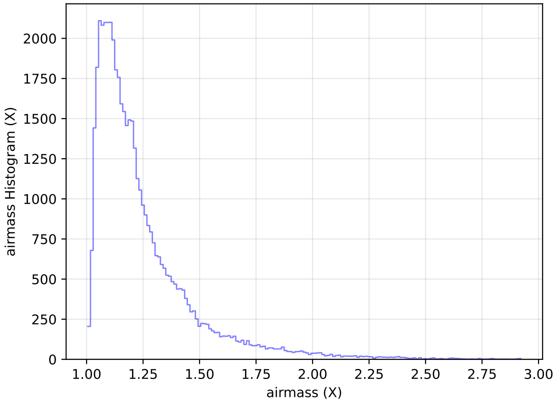
mw_roll_all_v3.3_10yrs Yr 1 y band: airmass Histogram
