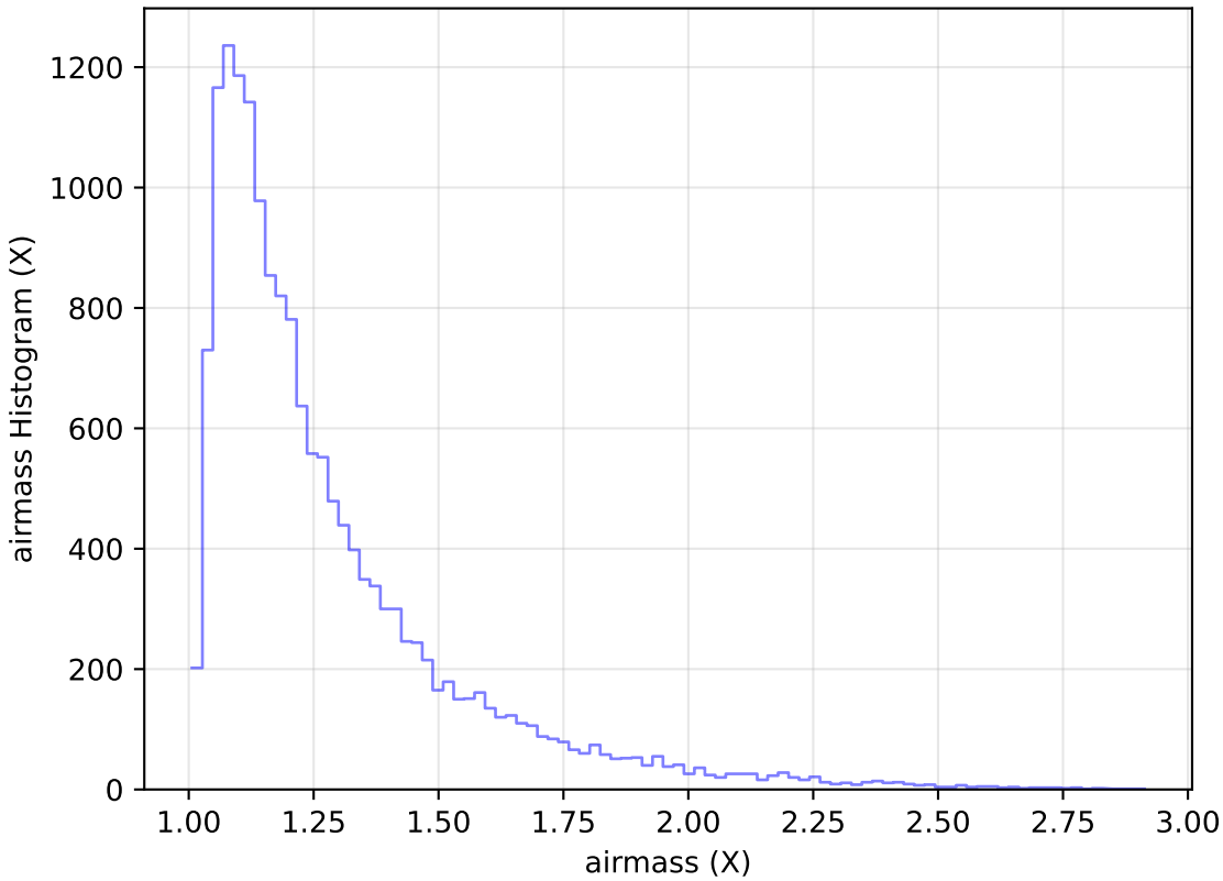
mw_roll_all_v3.3_10yrs Yr 1 u band: airmass Histogram
