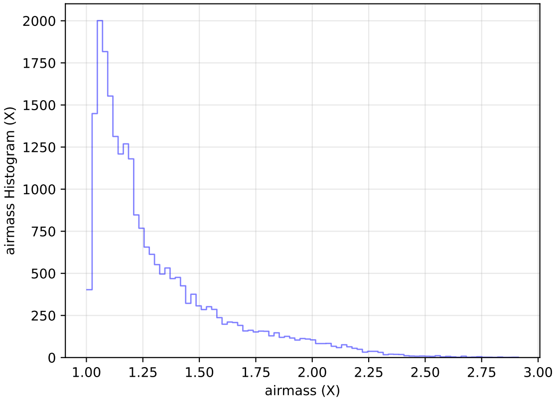
mw_roll_all_v3.3_10yrs Yr 1 g band: airmass Histogram
