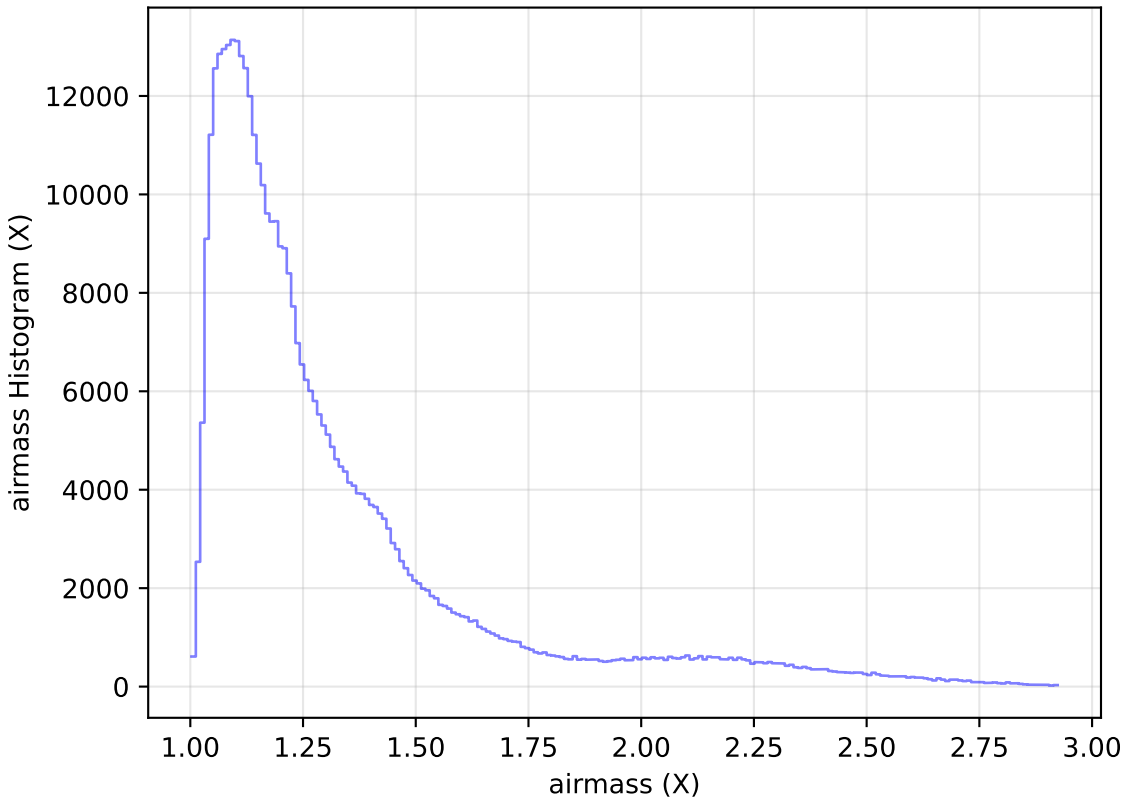
mw_roll_all_v3.3_10yrs WFD z band: airmass Histogram
