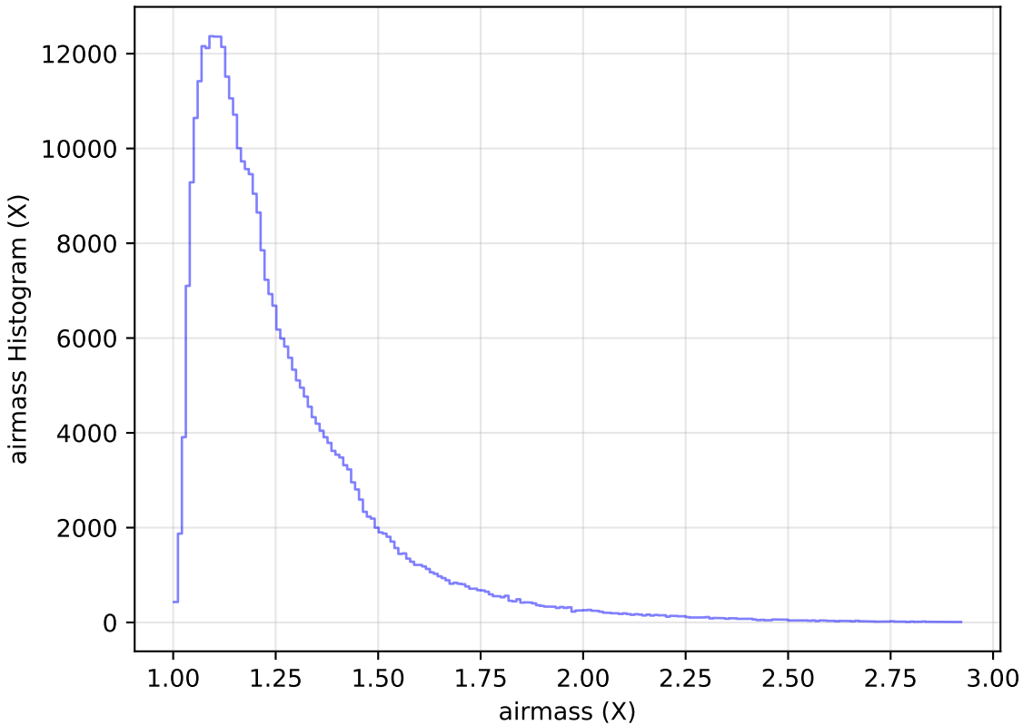
mw_roll_all_v3.3_10yrs WFD y band: airmass Histogram
