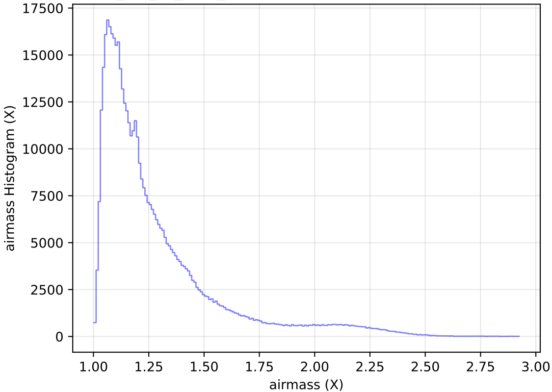
mw_roll_all_v3.3_10yrs WFD r band: airmass Histogram
