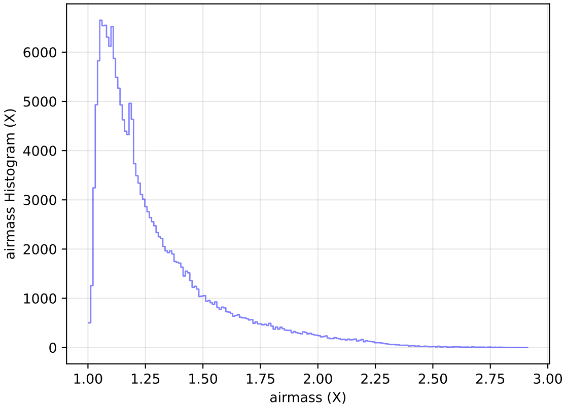
mw_roll_all_v3.3_10yrs WFD g band: airmass Histogram
