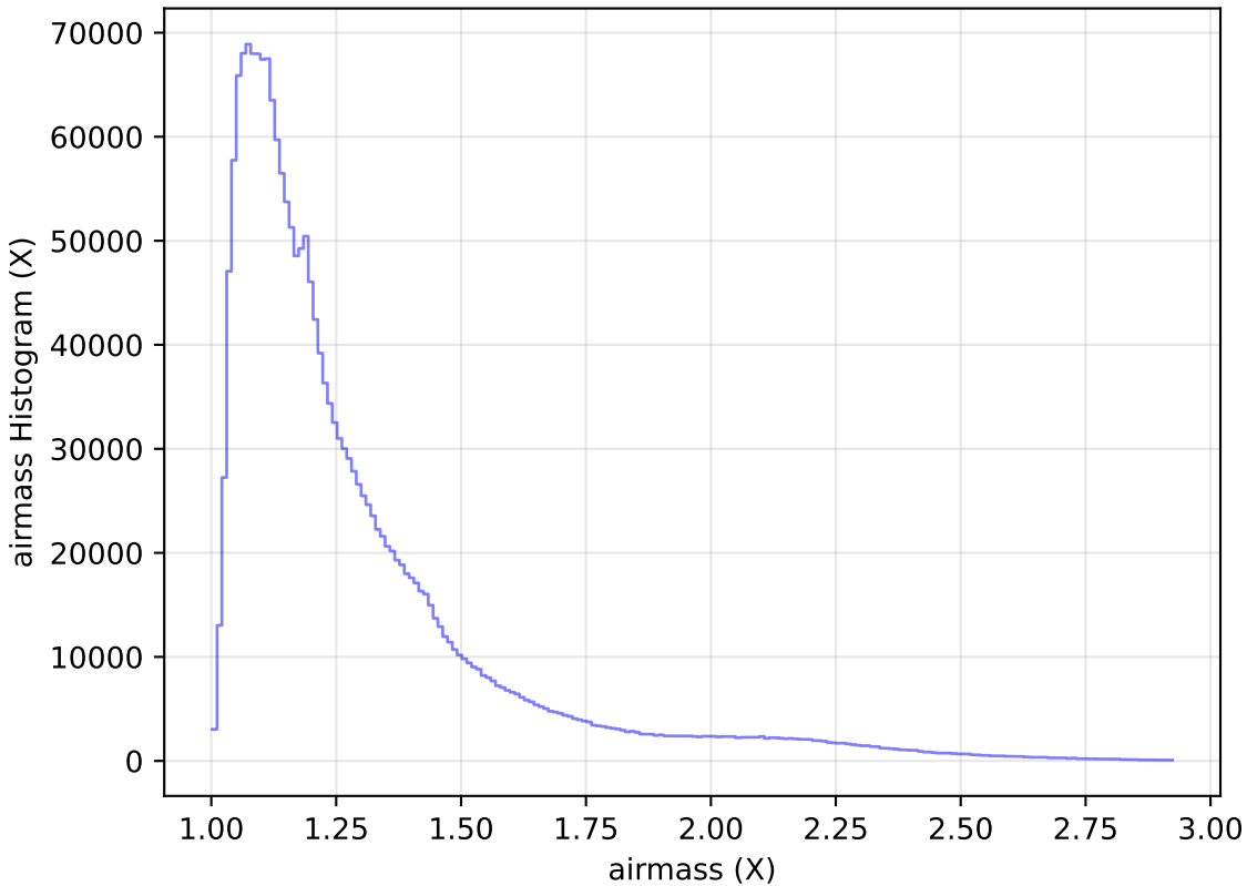
mw_roll_all_v3.3_10yrs WFD all bands: airmass Histogram
