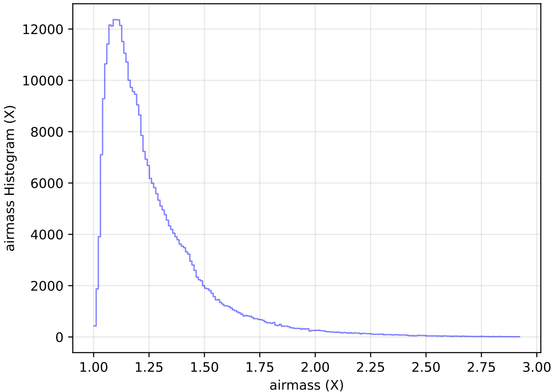
mw_roll_all_v3.3_10yrs All sky y band: airmass Histogram
