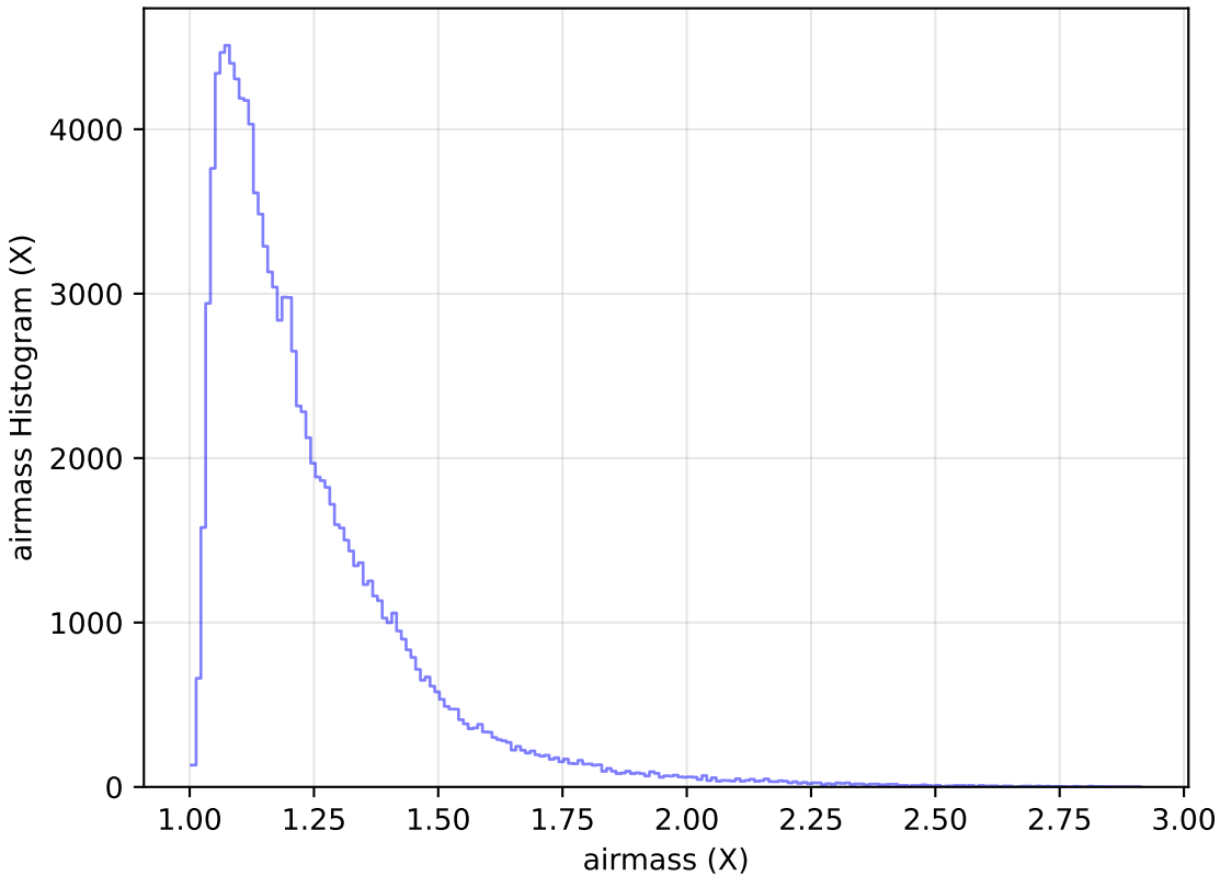
mw_roll_all_v3.3_10yrs All sky u band: airmass Histogram
