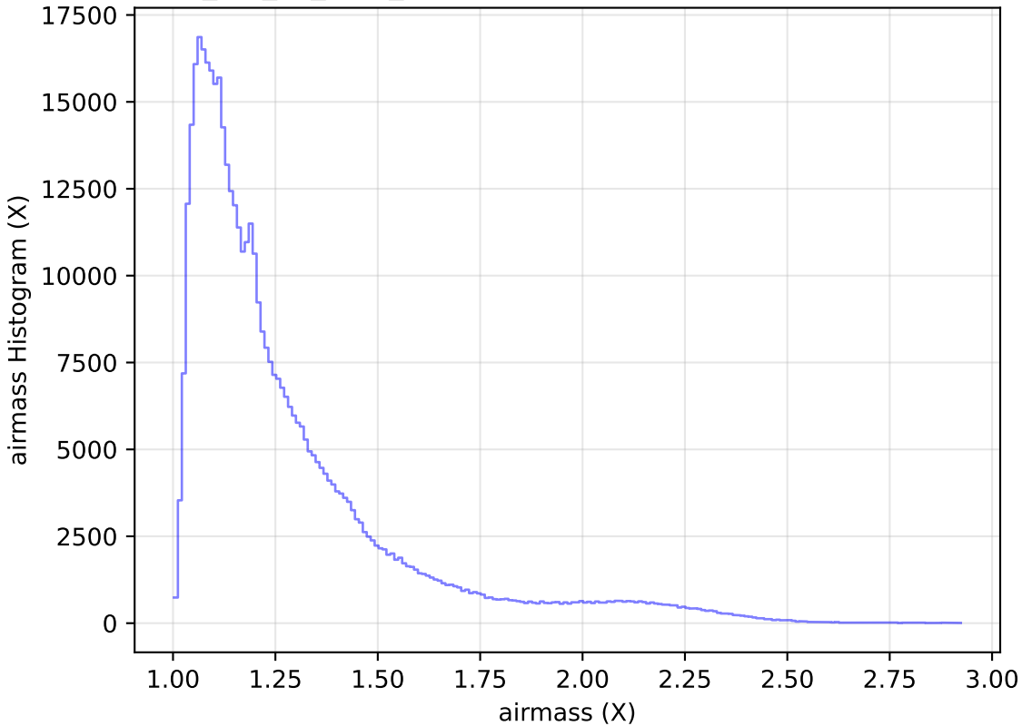
mw_roll_all_v3.3_10yrs All sky r band: airmass Histogram
