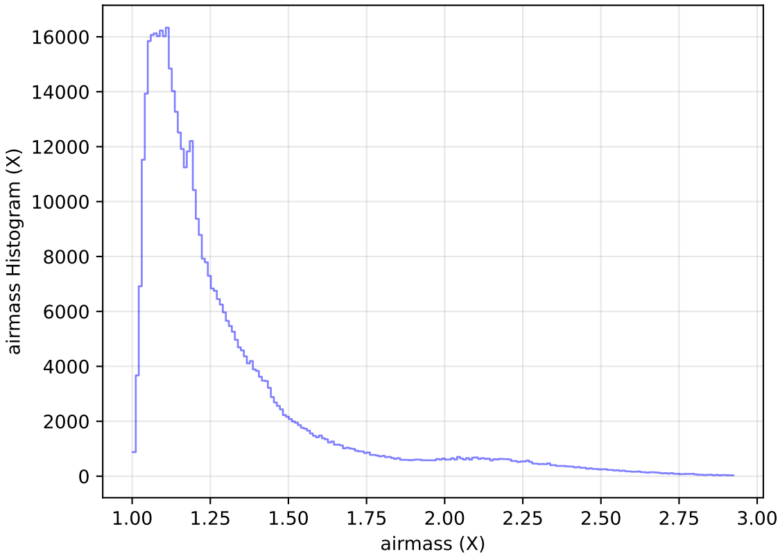
mw_roll_all_v3.3_10yrs All sky i band: airmass Histogram
