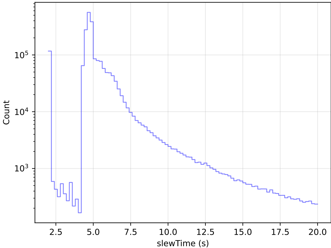
mw_roll_all_v3.3_10yrs All visits: Zoom Slew Time Histogram
