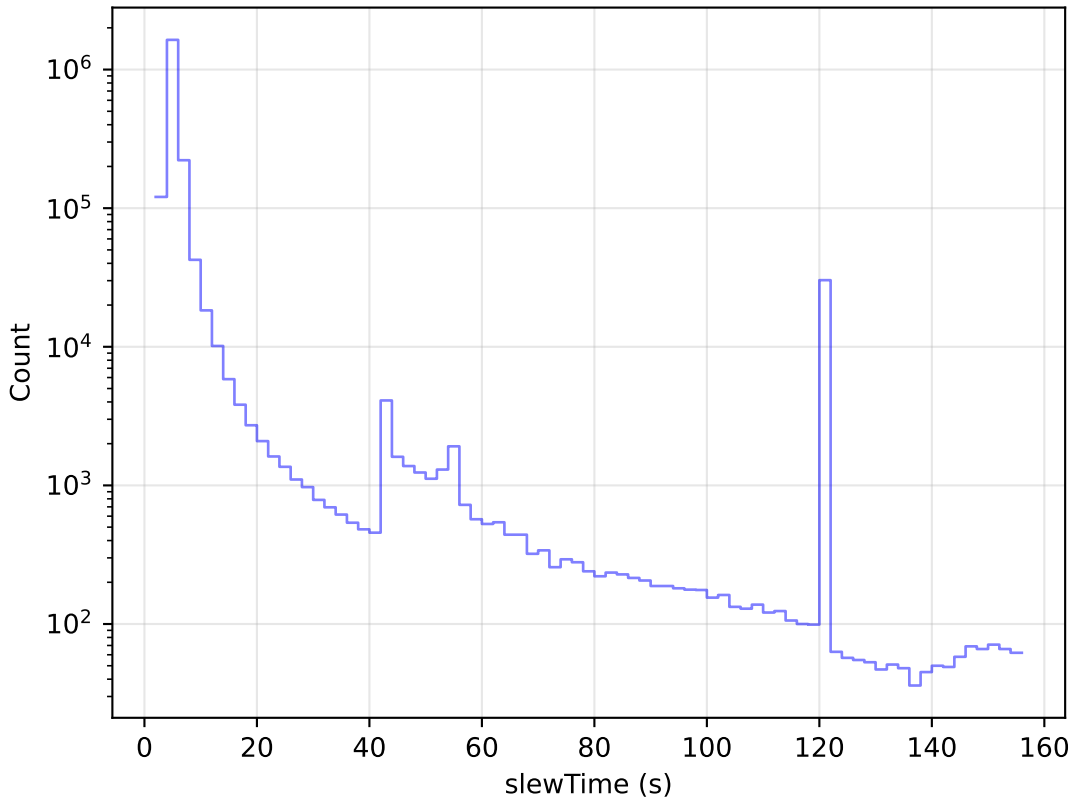
mw_roll_all_v3.3_10yrs All visits: Slew Time Histogram
