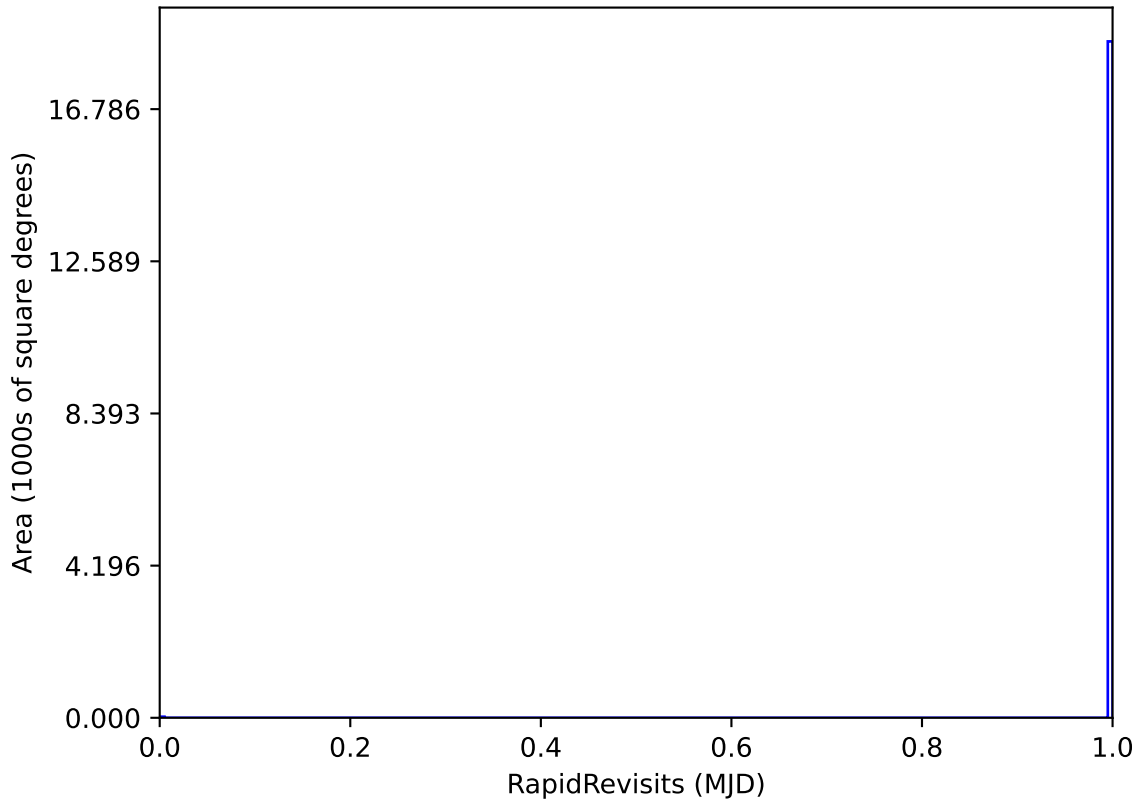
mw_roll_all_v3.3_10yrs WFD: RapidRevisits
