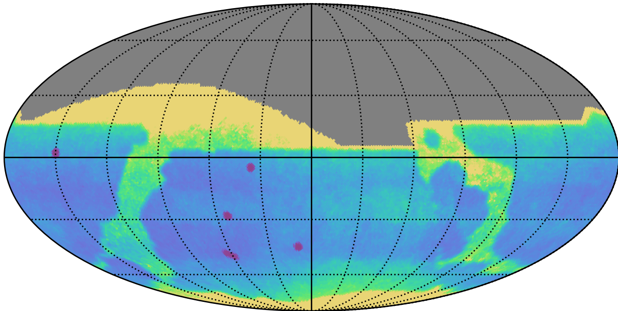
mw_roll_all_v3.3_10yrs All sky: Proper Motion Uncert @ 24.0
